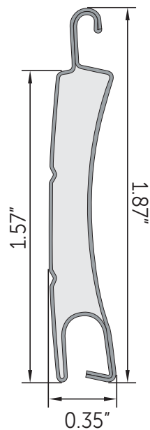
Shutter Dimension Diagram
