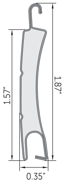
Shutter Dimension Diagram
