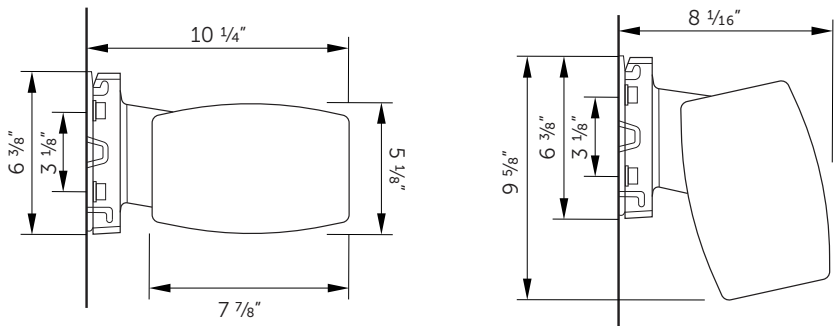
Wall Bracket
