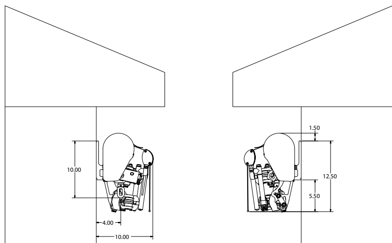
Awning Drop Arm Closed - Side View
