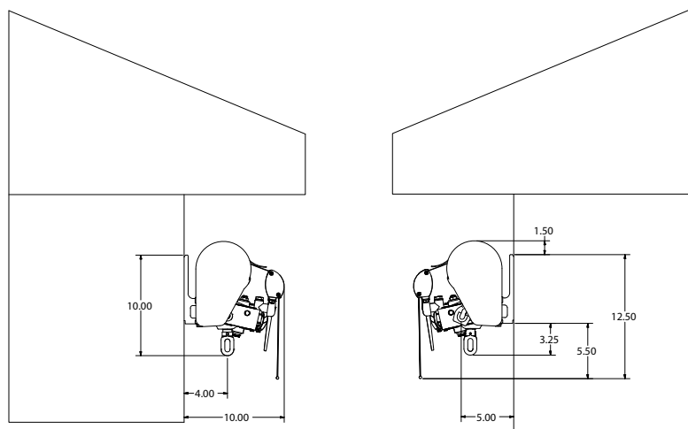
Awning Closed - Side View
