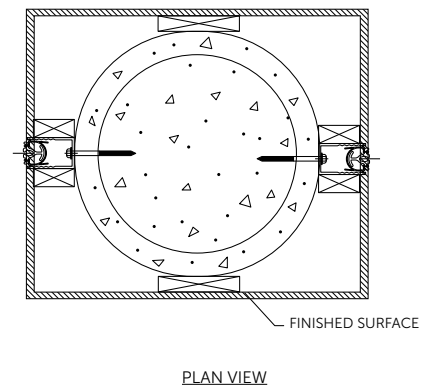
SECTION "b-b" PARTIAL PLAN VIEW OF ROLL DOWN SCREEN ASSEMBLY CONNECTION TO COLUMNS-FLANGE MOUNT
