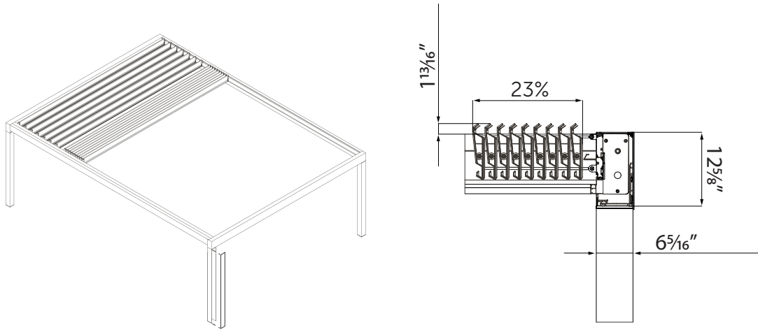
Retracting System
