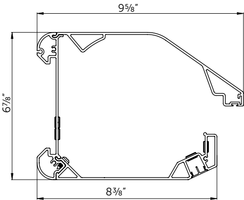
Low Support Bracket - Standard
