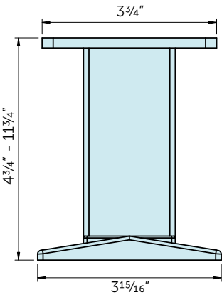
Extended Support Bracket (to clear obstacles)
