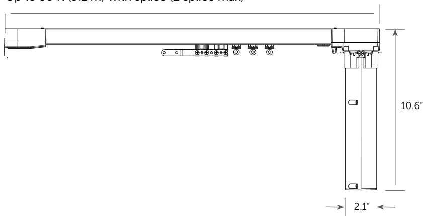
Front view (single track, right draw)
