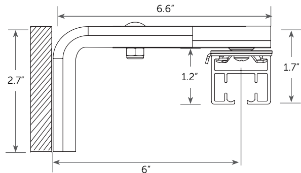
Maximum Extension
