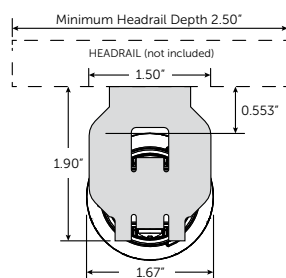
Roller 64 Bracket
