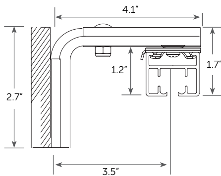
Minimum Extension
