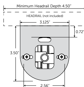
Roller 100 & Roller 150 Bracket
