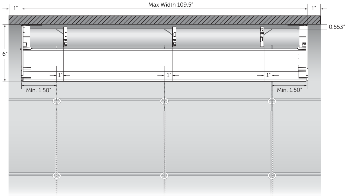
Fabric Panel and Lift Cord Placement
