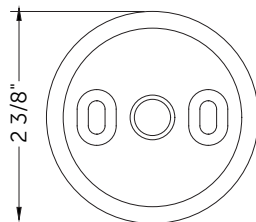
R1 Dimensions - Front Face
