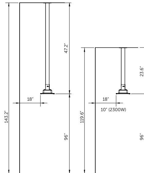
Ceiling Pole Clearance
