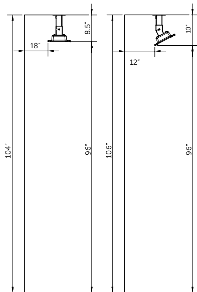
Ceiling Mount Clearance
